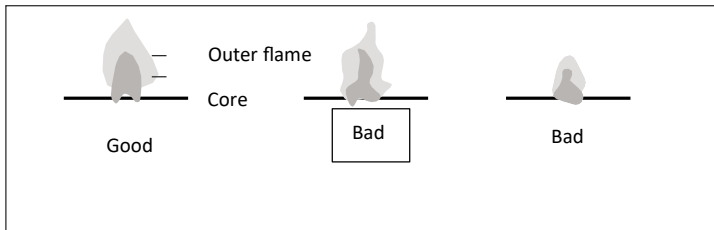
Air damper
